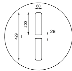
Free Standing Feet FIX screen
